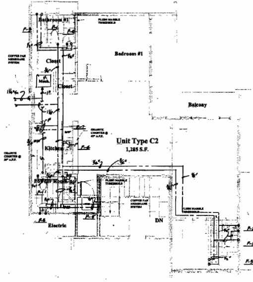
PLUMBING WATER & GAS LAYOUT UNIT# 403 SCALE: 1/4"=1'-0"
