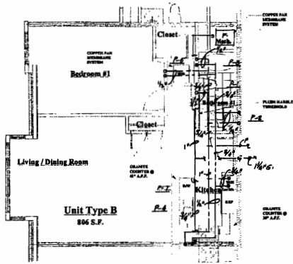
PLUMBING WATER & GAS LAYOUT UNITS# 102, 104, 202, 204, 302, 304, 402, 404 SCALE: 1/4"=1'-0"
