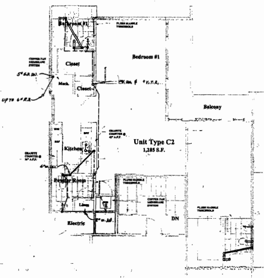
PLUMBING WASTE & VENT LAYOUT UNITS# 403 SCALE: 1/4"=1'-0"
