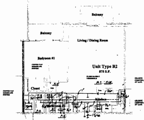
PLUMBING WATER & GAS LAYOUT UNITS# 107, 207 SCALE: 1/4"=1'-0"
