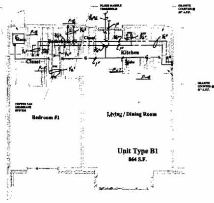
PLUMBING WATER & GAS LAYOUT UNITS# 108, 208, 308 SCALE: 1/4"=1'-0"
