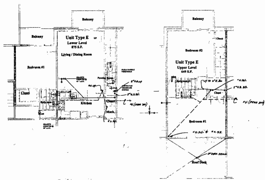
PLUMBING WASTE & VENT LAYOUT LOWER LEVEL UNIT #307 SCALE: 1/4"=1'-0"
